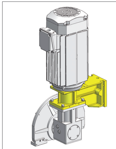
Customized support
